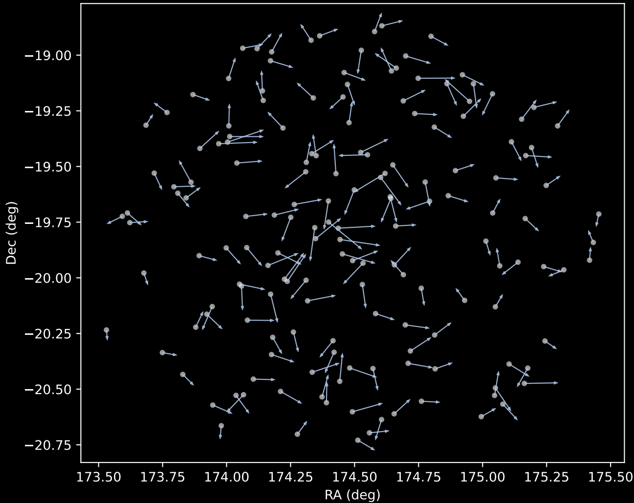
GALAH DR4 Cluster 1 Proper Motion Vectors (n=162)
