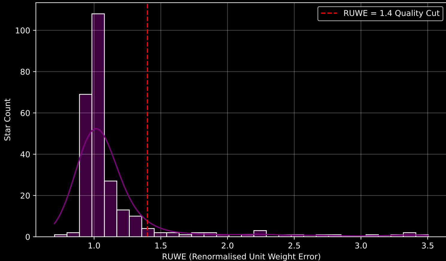
GALAH DR4 Field [676] RUWE Distribution (n= 257)
