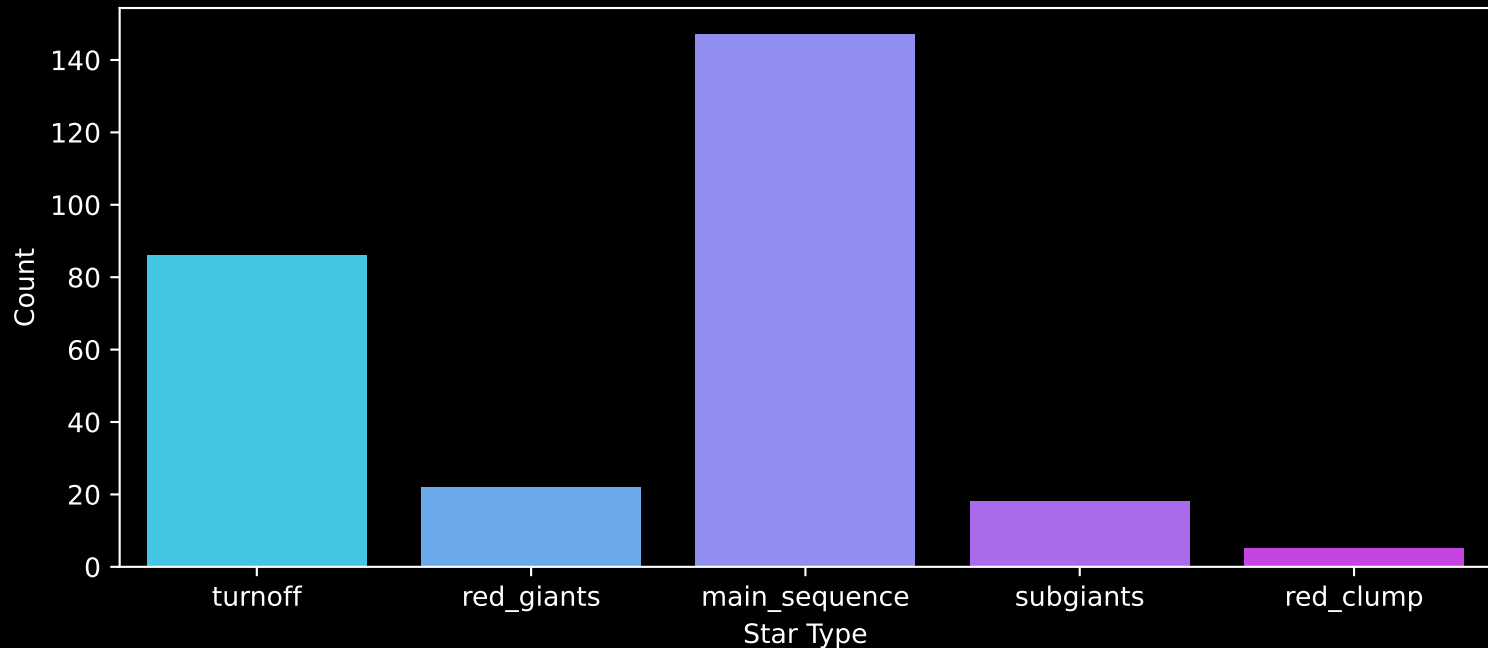
GALAH DR4 Field: [676] Count plot of Star Type
